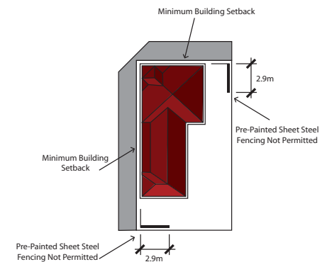
Figure 2.16.8. Pre-painted sheet steel fencing on common lot boundaries
