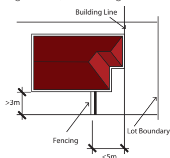
Figure 2.16.9. Return fencing permitted to be constructed from pre-painted sheet steel
