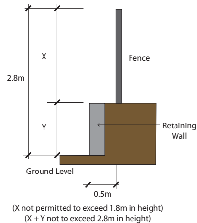
Figure 2.16.7. Lot fencing abutting a road reserve on a retaining wall
