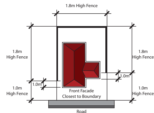
Figure 2.16.5. Common boundary fencing
